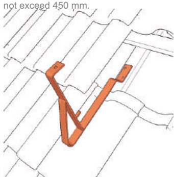
Type A Installed with an additional batten
