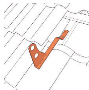
Type A Attached with additional batten
